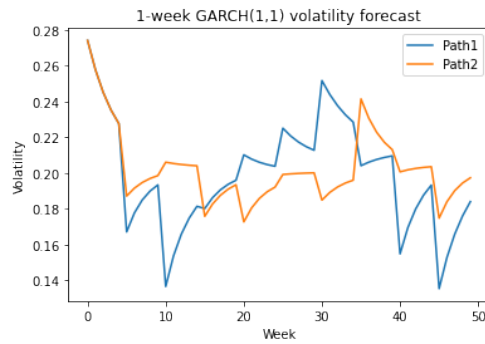
Figure 19: Weekly volatility forecast.
