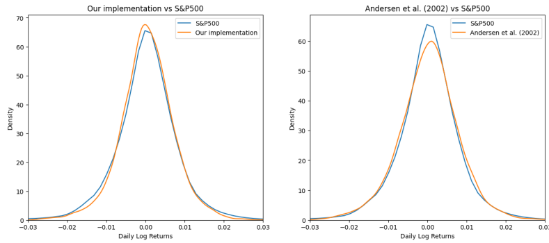
Figure 12: Comparison of calibrated Bates models and S&P500 densities.
