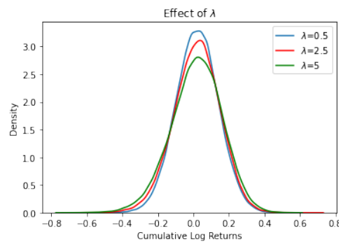
Figure 3: Effect of \lambda on returns.
